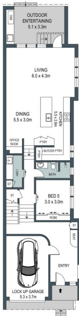
GROUND FLOOR
