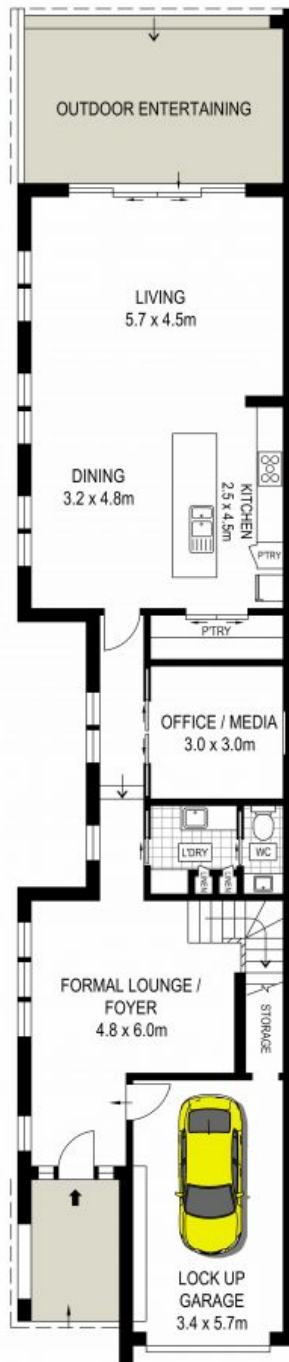
GROUND FLOOR
