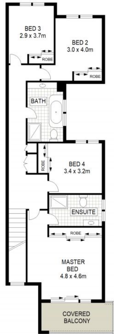
FIRST FLOOR
