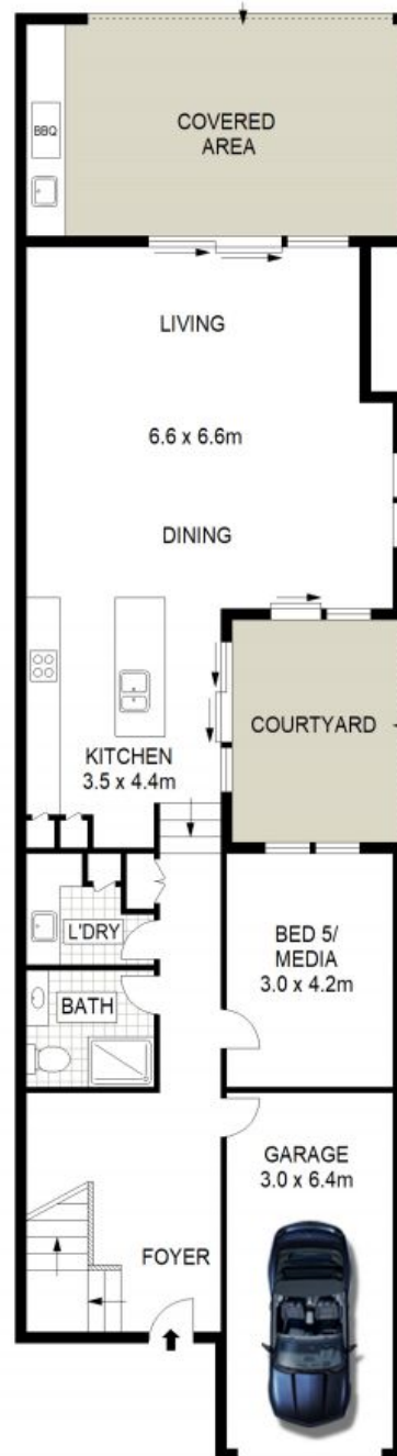
GROUND FLOOR
