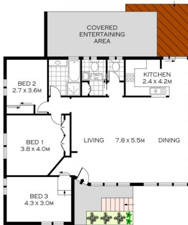
ELEVATED GROUND FLOOR
