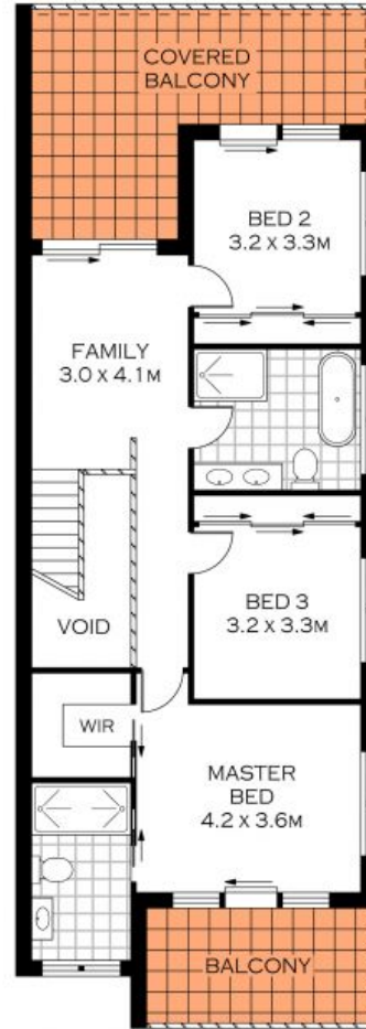
FIRST FLOOR
