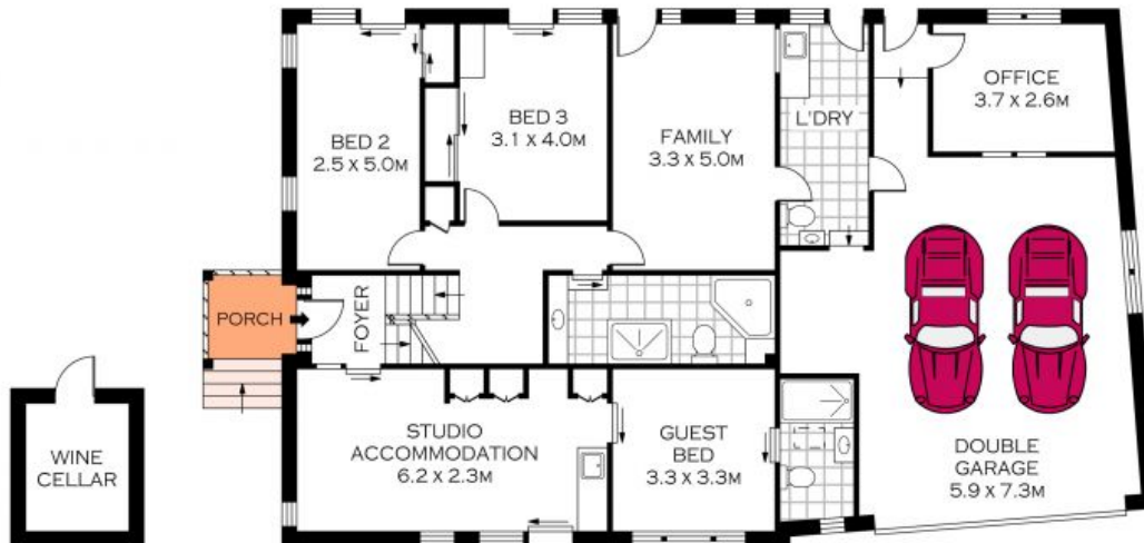
GROUND FLOOR
