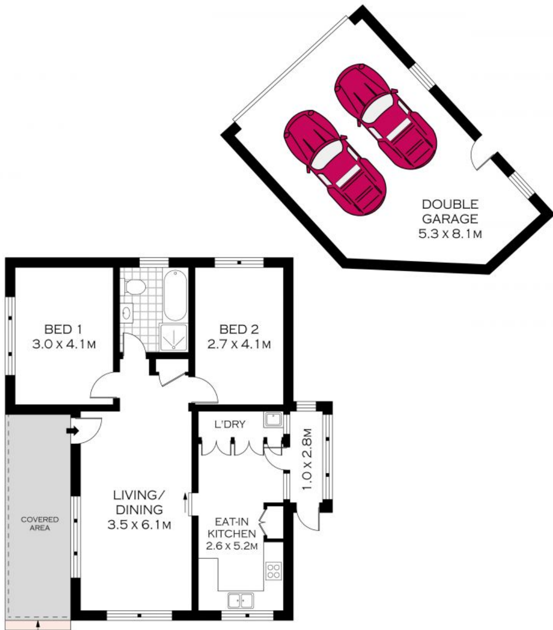
GROUND FLOOR
