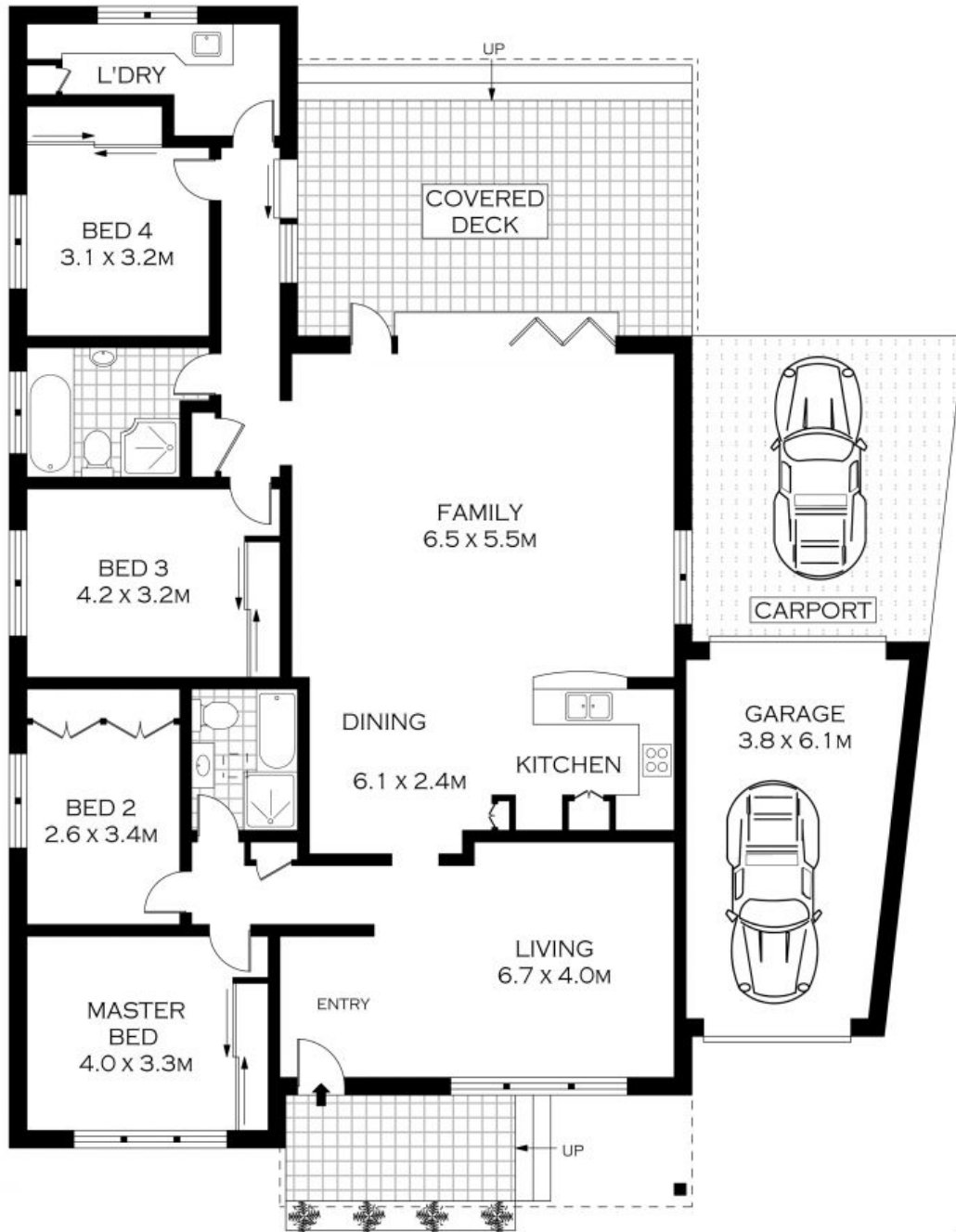
GROUND FLOOR
