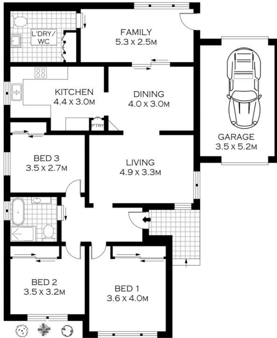
FLOOR PLAN
