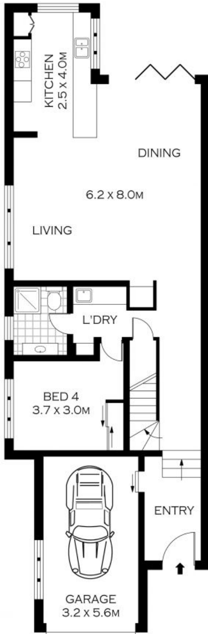
GROUND FLOOR
