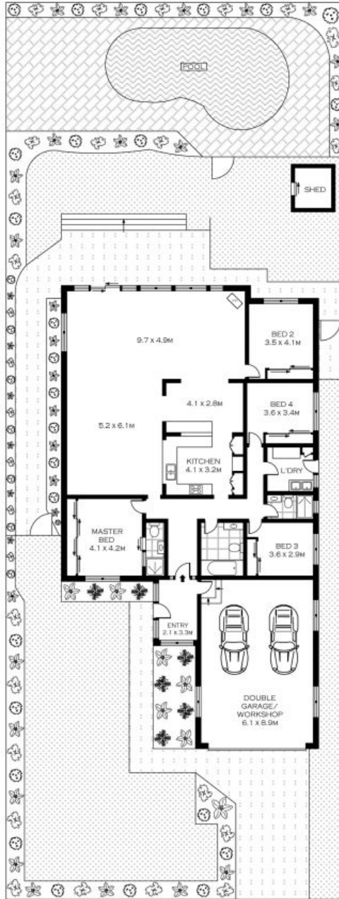
GROUND FLOOR
